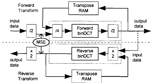
Fig. 5: Data Arrangement for a 2-D DCT
