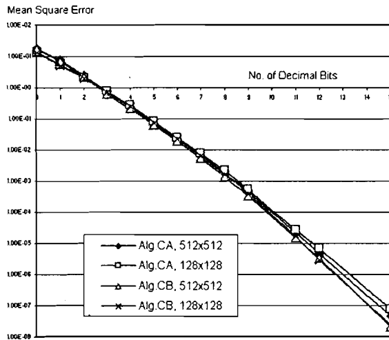
Fig. 9: MSE Performance of Algorithms CA and CB
