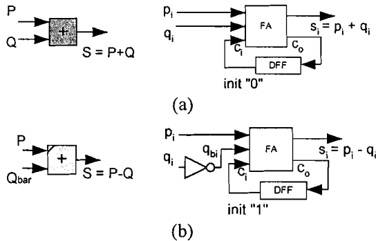
Fig. 6: (a) A Bit-Serial Adder (b) A Bit-Serial Subtractor
