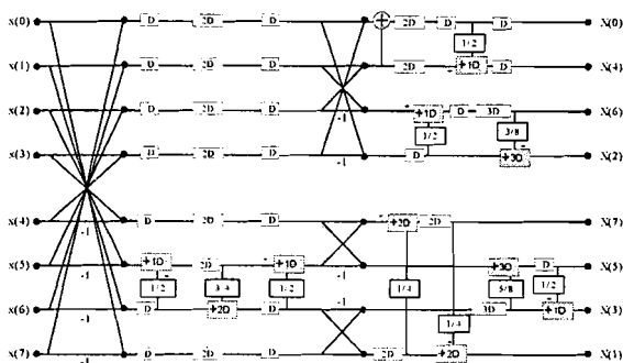
Fig. 8: An Architecture With Bit Slicing Technique
